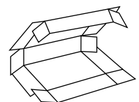
Name: FEFCO STYLE 0421 Description: Folding box with locking sides
